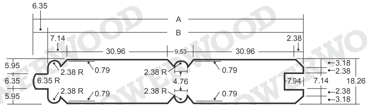
1" X 4" E & CB Partition
